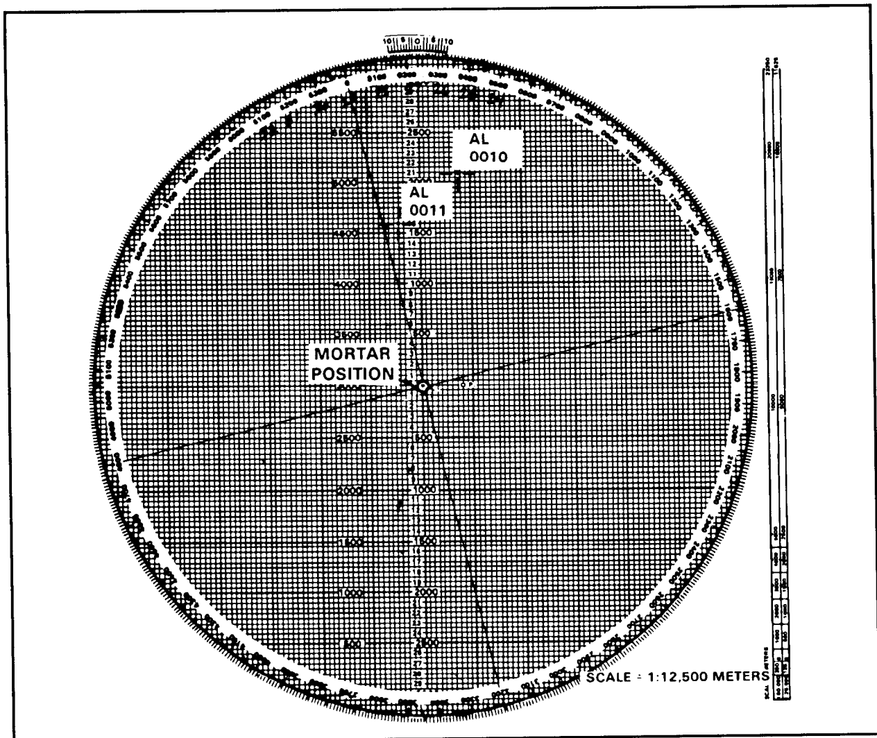
Figure 12-20. Observed chart.
